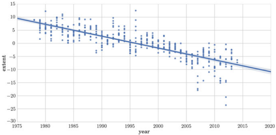
Fig. 6.4 Regression model fitting sea ice extent data for all months by year using lmploT
